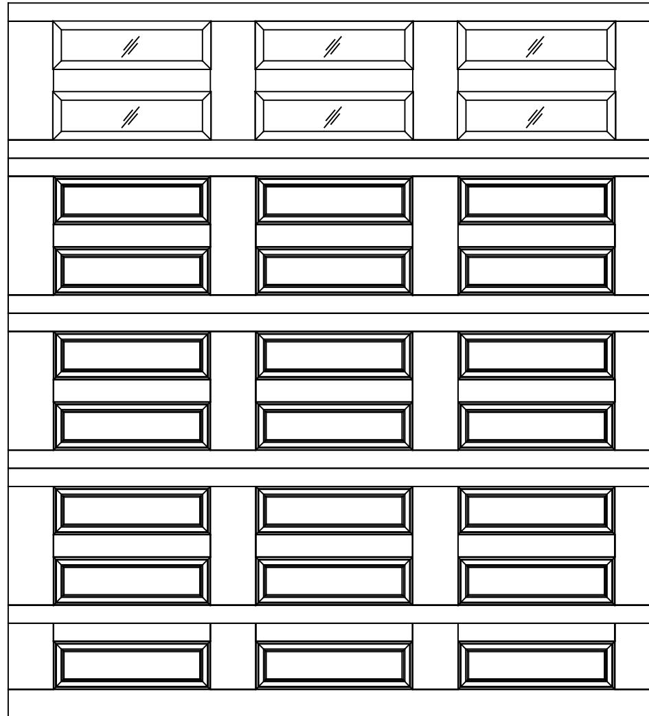
9x10 9800 HRP DESIGN 5 SECTION/3 PANEL PLAIN GLAZED TOP SECTION SHOWN CONSISTS OF: (4) 25.73" & (1) 16.00" SECTIONS
