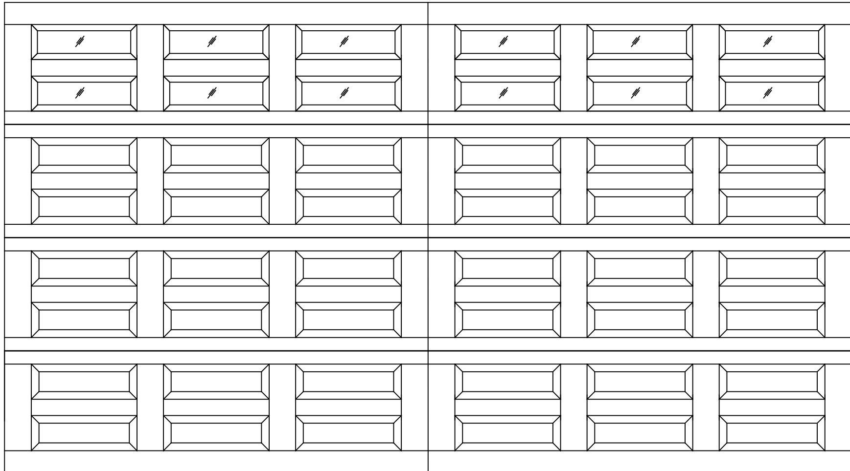
16x9 9800 HRP 4 SECTION/6 PANEL PLAIN GLAZED TOP SECTION SHOWN CONSISTS OF: (2) 25.73" & (2)27.73" SECTIONS
