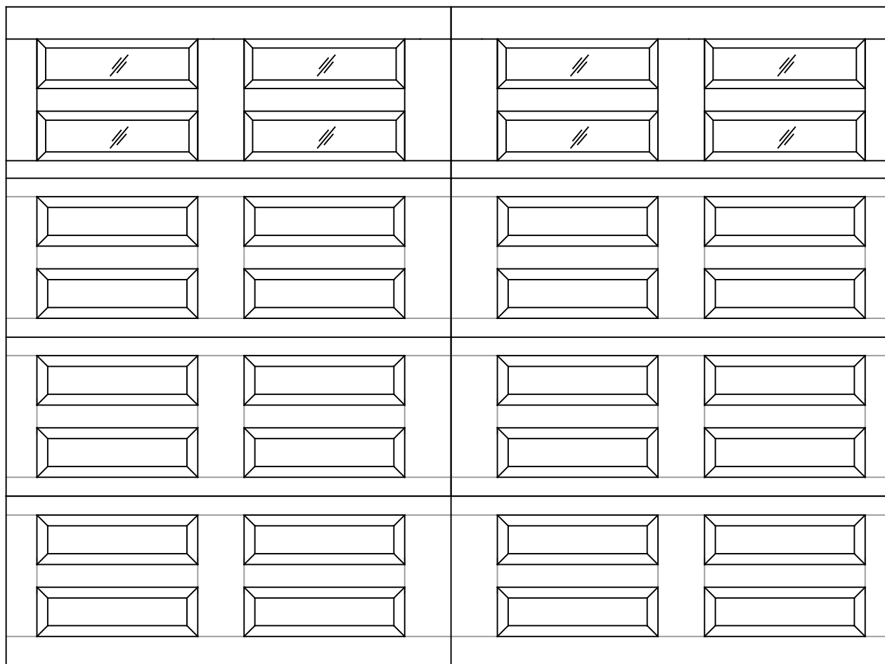
12 x 9 9800 HRP DESIGN 4 SECTION, 4 PANEL PLAIN GLAZED TOP SECTION SHOWN CONSISTS OF: (2) 27.73" & (2) 25.73" SECTION
